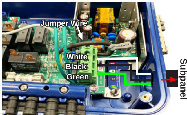
Field Converted 115V 30 Amp Control Box
