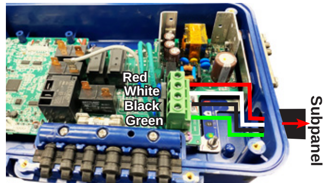
Field Converted 115/230V Control Box
